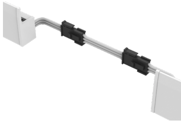
Dry Continuous Connector (20/3 Gauge Wire) (A8-ZYPO-RPI-CC-SFF-DRY-X) X = Specify Length, 3" Default
