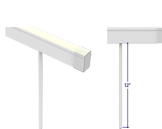
Back of Fixture Feed Power Connector for HB Lightstrip (20/2 Gauge Wire) (A8-ZUFI-FLX-PC-BFF-HB-X-12") X = Specify Listing: Dry (DRY) or Wet (WET)
