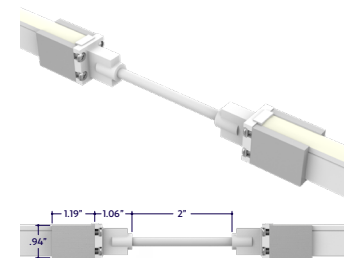
Jumper Cable for HB Lightstrip (20/2 Gauge Wire) (A8-ZUFI-FLX-JC-HB-X-2") X = Specify Listing: Dry (DRY) or Wet (WET)
