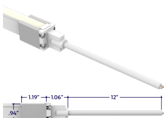
End Feed Power Connector for HB Lightstrip (20/2 Gauge Wire) (A8-ZUFI-FLX-PC-EF-HB-X-12") X = Specify Listing: Dry (DRY) or Wet (WET)
