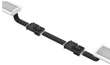
Dry Continuous Connector with Black Jacket (20/3 Gauge Wire) (A8-ZUDA-RCL-CC-BFF-DRY-BK-X) X = Specify Length, 3" Default
