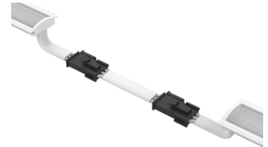
Dry Continuous Connector with White Jacket (20/3 Gauge Wire) (A8-ZUDA-RCL-CC-BFF-DRY-WH-X) X = Specify Length, 3" Default
