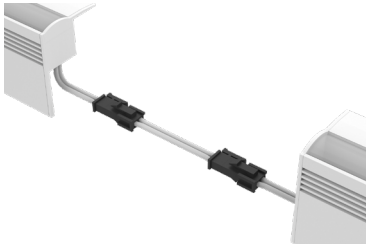
Dry Continuous Connector (20/2 Gauge Wire) (A8-ZIGY-RCP-CC-BFF-DRY-X) X = Specify Length, 3" Default
