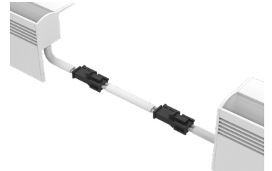
Dry Continuous Connector with White Jacket (20/2 Gauge Wire) (A8-ZIGY-RCP-CC-BFF-DRY-WH-X) X = Specify Length, 3" Default
