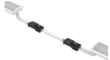
Dry Continuous Connector with White Jacket (20/2 Gauge Wire) (A8-ZIGY-RCL-CC-BFF-DRY-WH-X) X = Specify Length, 3" Default
